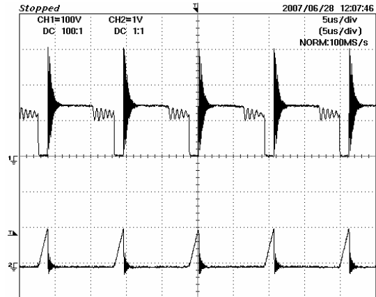
Figure 15 – 90 VAC, V_{out}= 2.3\text{ V} , I_o= 3\text{ A} Upper: V_{DRAIN} , 100 V Lower: I_{DRAIN} , 1.0 A / div, 5 \mu\text{s} / div.
