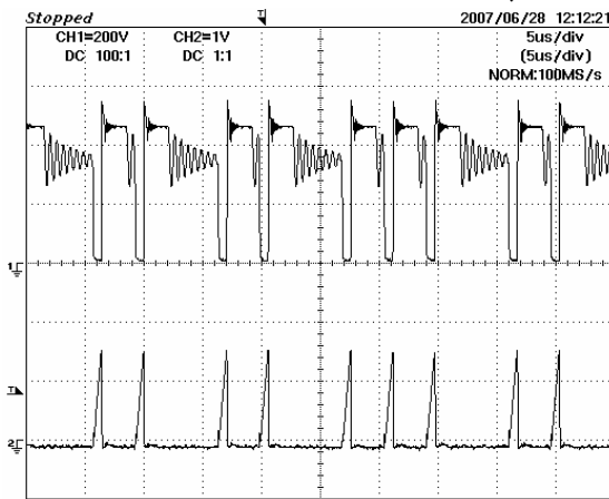
Figure 16 – 230 VAC, V_{out}= 12\text{ V} , I_o= 3\text{ A} Upper: V_{DRAIN} , 100 V Lower: I_{DRAIN} , 1.0 A / div, 5 \mu\text{s} / div.
