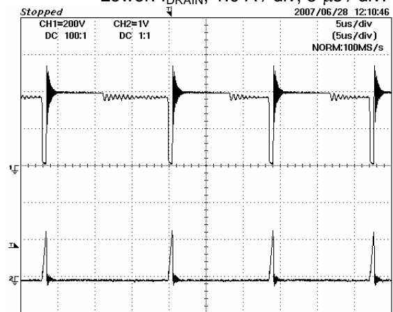
Figure 17 – 230 VAC, V_{out}= 2.3\text{ V} , I_o= 3\text{ A} Upper: V_{DRAIN} , 100 V Lower: I_{DRAIN} , 1.0 A / div, 5 \mu\text{s} / div.
