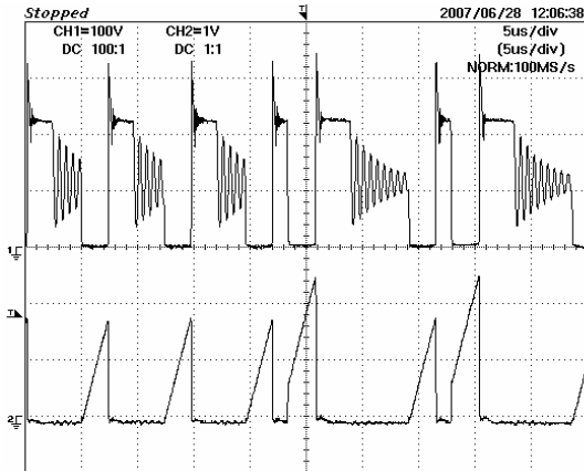
Figure 14 – 90 VAC, V_{out}= 12\text{ V} , I_o= 3\text{ A} Upper: V_{DRAIN} , 100 V Lower: I_{DRAIN} , 1.0 A / div, 5 \mu\text{s} / div.
